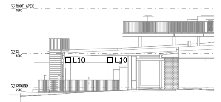
SOUTH EXTERNAL BUILDING ELEVATION SCALE 1:200
