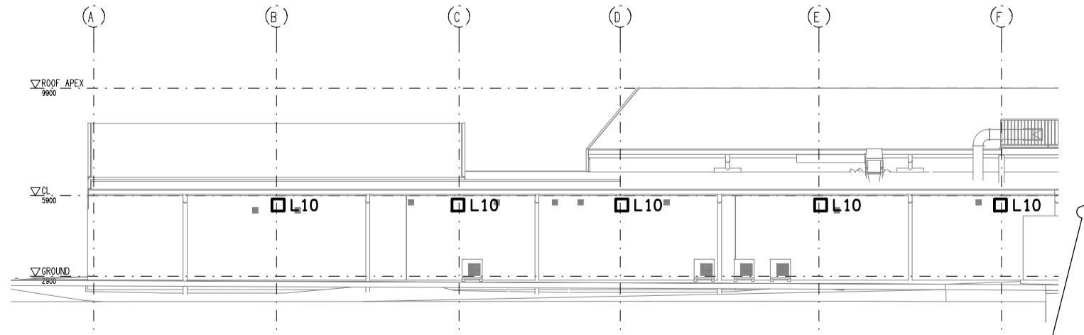
WEST EXTERNAL BUILDING ELEVATION SCALE 1:200
